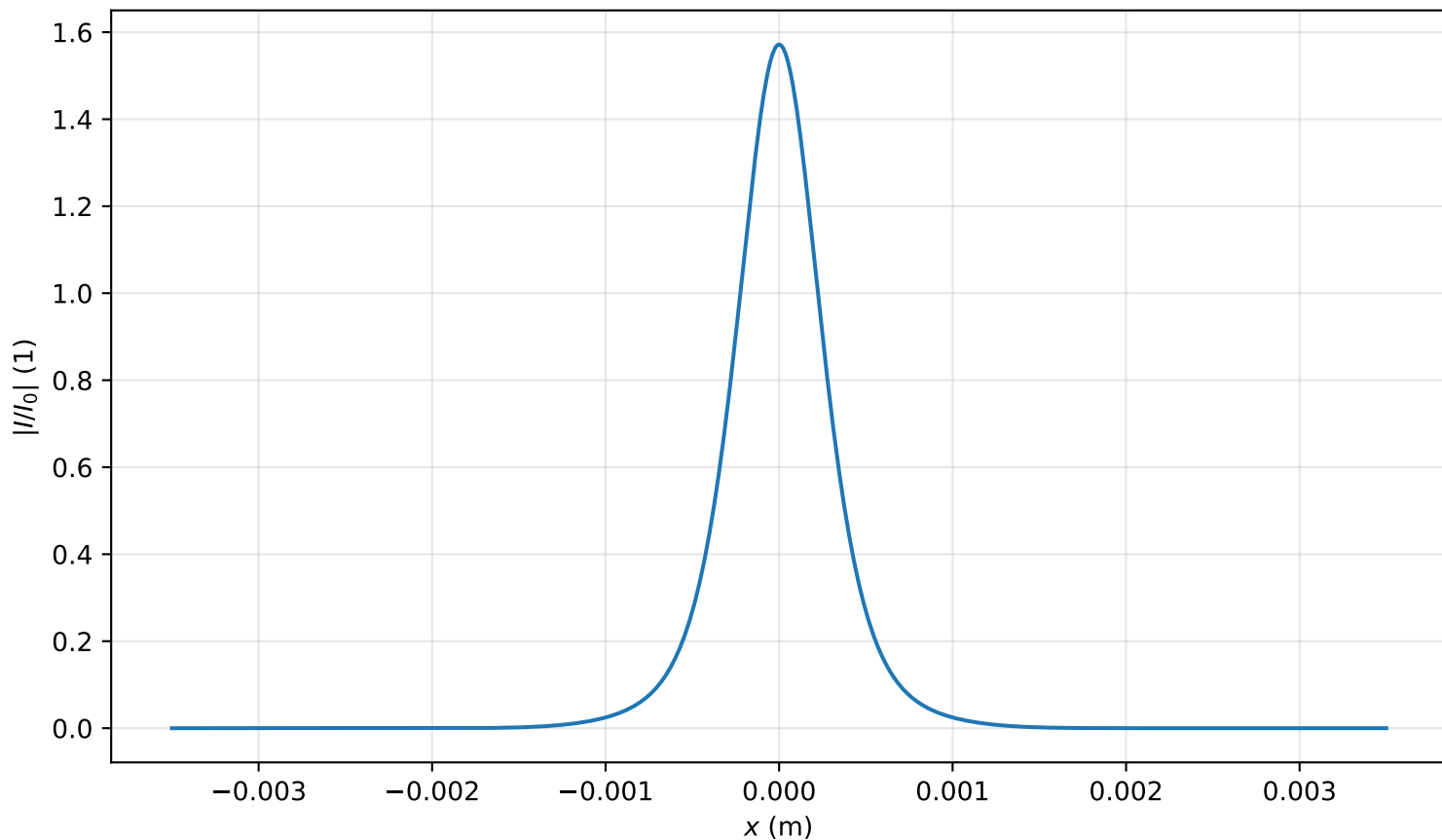
Intensity profile I(x, y = 0, z = 1.513m)/I_0 , P_{in}=0.9P_{cr} , artificial time
